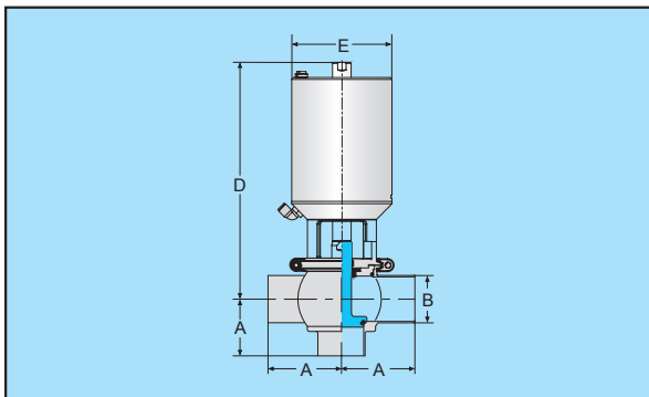
F型气动单座阀
