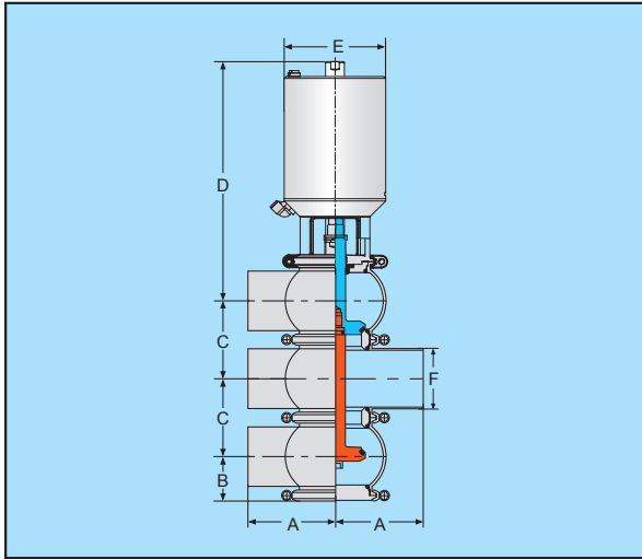
B型气动分流阀
