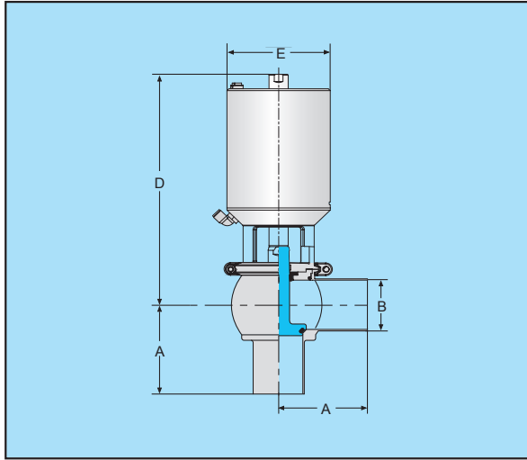
L型气动单座阀
