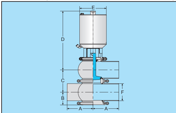
F型气动单座阀
