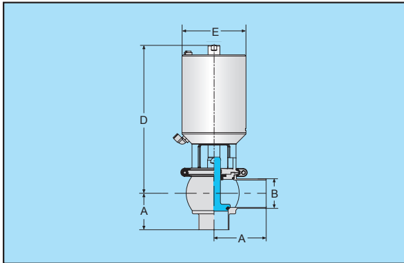
T型气动单座阀
