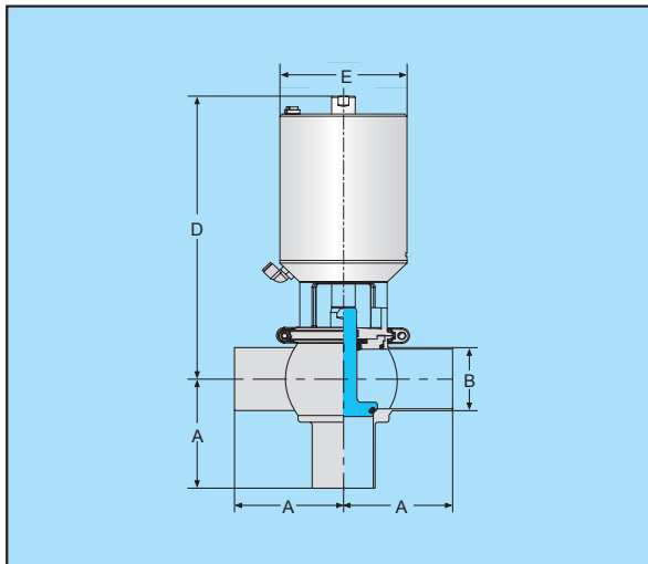
T型气动单座阀
