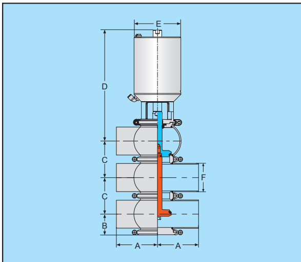
B型气动分流阀
